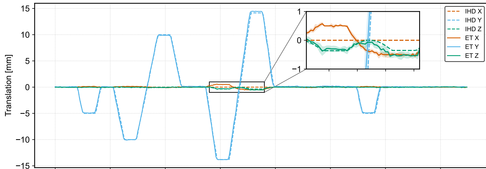
ExacTrac surface outputs vs. IHD (with moving axes: All axes)
